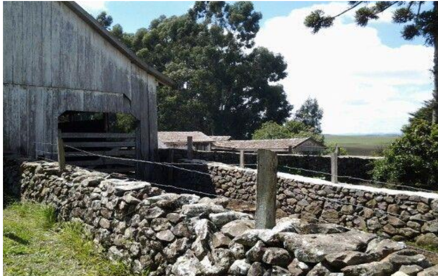
Fig. 6- Taipas e Aramados – Lages/SC
